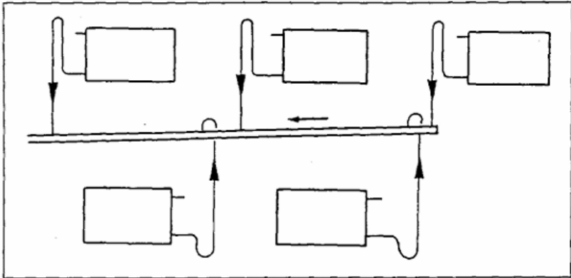
5. Coolers at different heights and with a common suction pipe.
